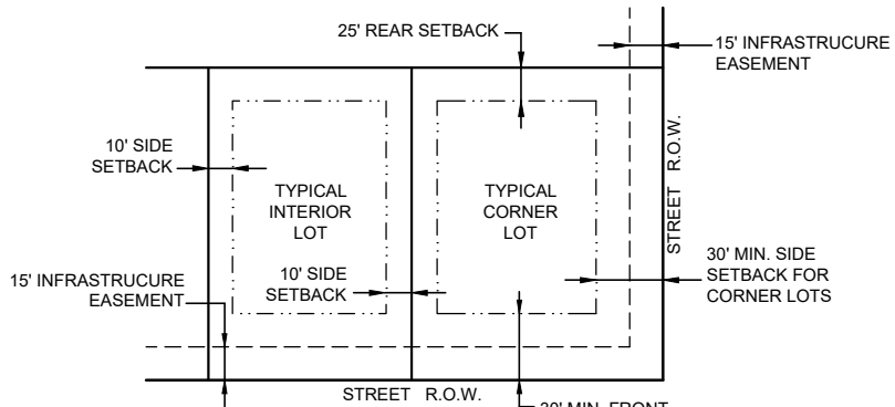
TYPICAL LOT DETAIL WITH SETBACKS
